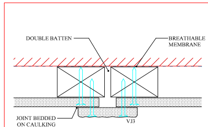
5A CONTINUOUS VERTICAL JOINT
