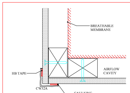
6A 90° EXTERNAL CORNER ANGLE
