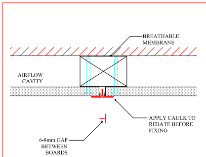
5 PLANK JOINT MOULDING
