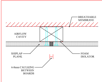
4 CAULKED JOINT
