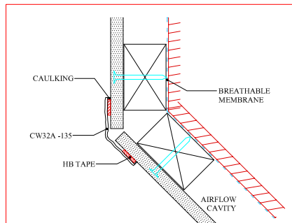
7A 135° EXTERNAL CORNER ANGLE
