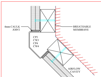
7 135° EXTERNAL CORNER POST
