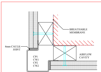
6 90° EXTERNAL CORNER POST
