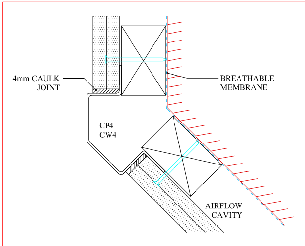
7 135° EXTERNAL CORNER POST
