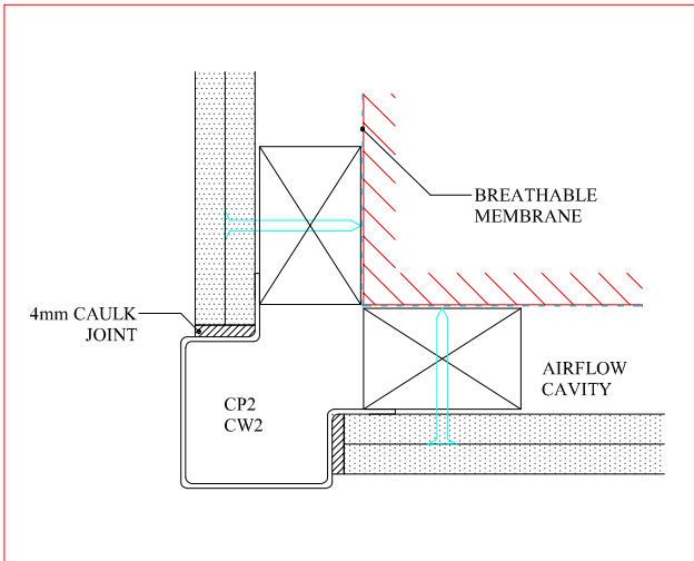
6 90° EXTERNAL CORNER POST
