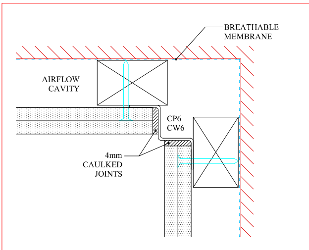
8 90° INTERNAL CORNER POST
