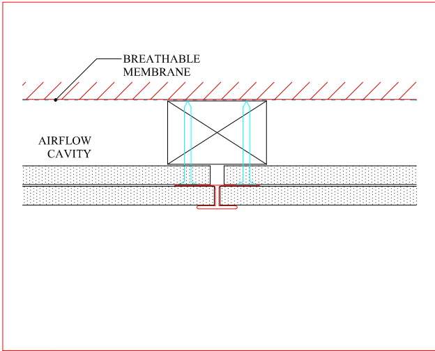
5 PLANK JOINT MOULDING
