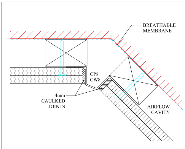
9 135° INTERNAL CORNER POST
